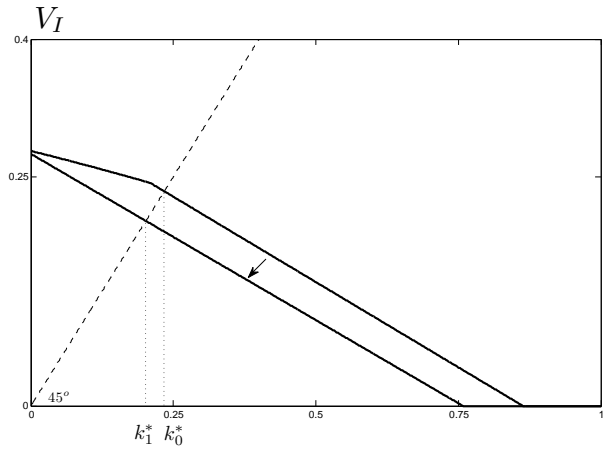
Figure 3: An Increase in \gamma When \lambda^* > \underline{\lambda}(\gamma)
