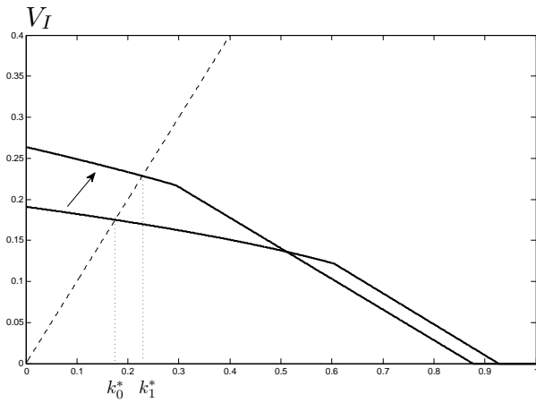
Figure 2: An Increase in \gamma When \lambda^* < \underline{\lambda}(\gamma)
