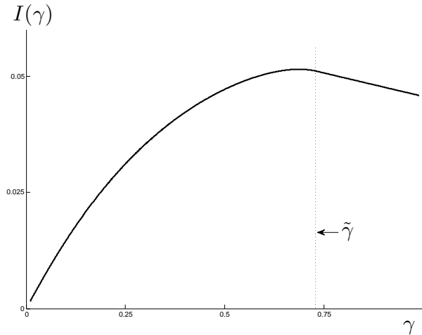
Figure 4: The Quantity of Information and Policy
