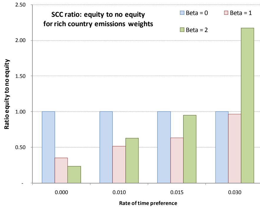
Figure 4. Ratio of SCC with to those without equity weighting where rich countries' consumptions are used as numéraire.
