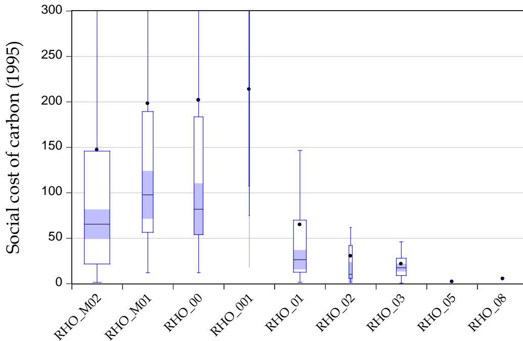
Figure 7. Boxplot of estimated social cost of carbon for different pure rates of time preference
