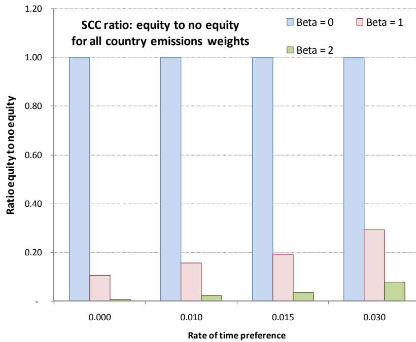
Figure 3. Ratio of SCC with to those without equity weighting where all countries' consumptions are used as numéraire. "Beta" is the assumed elasticity of the utility function.
