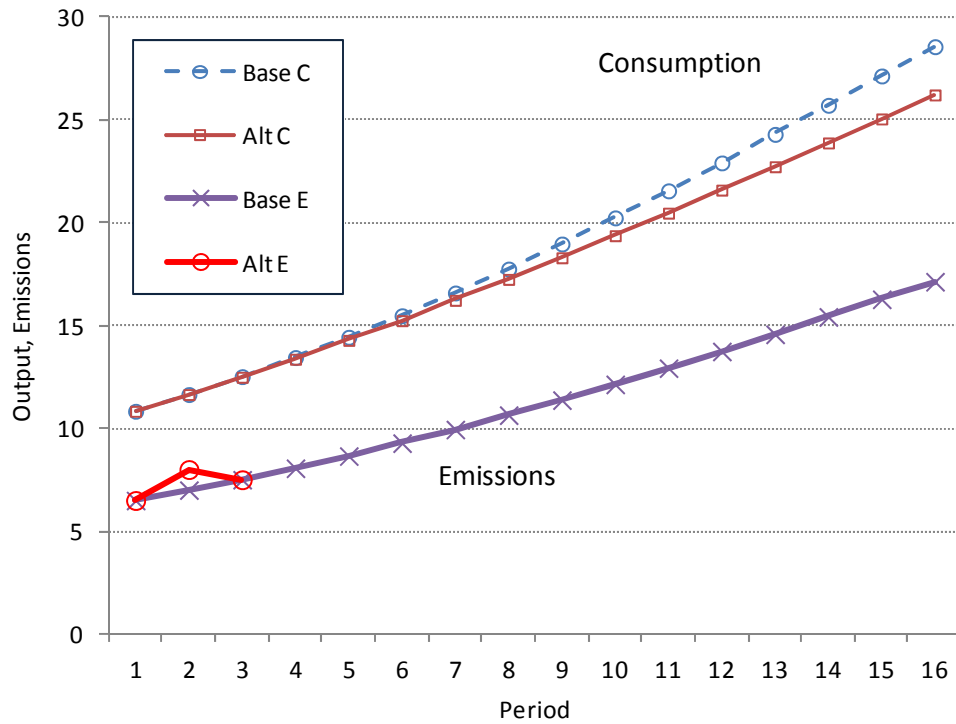
Figure 1. Illustration of calculation of social cost of carbon
