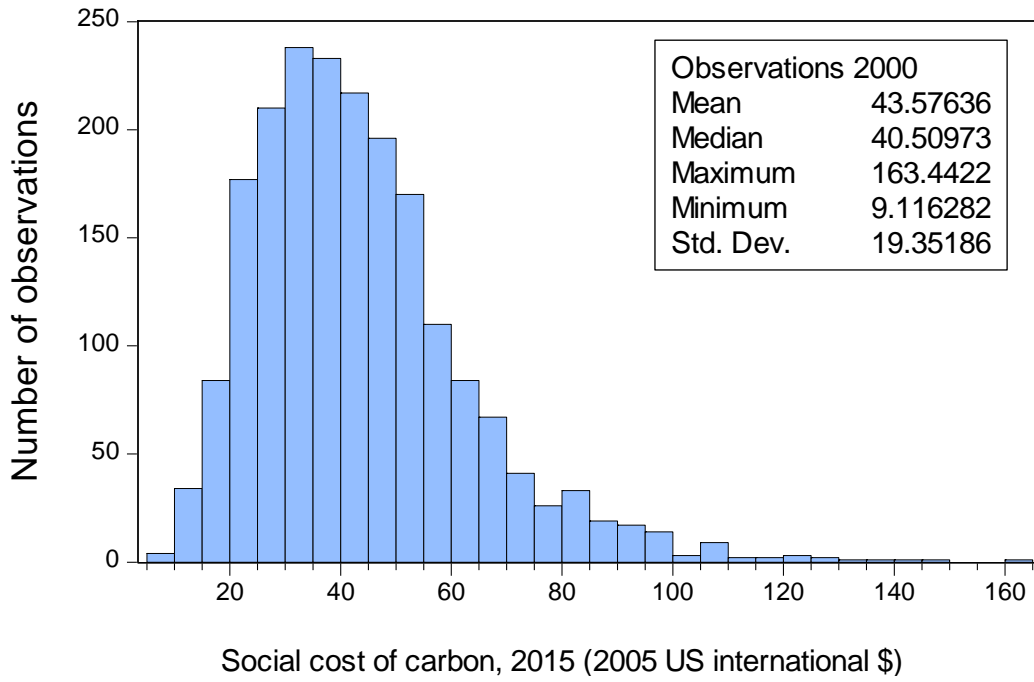
Figure 5. Distribution of the estimated SCC for 2015 in uncertainty runs
