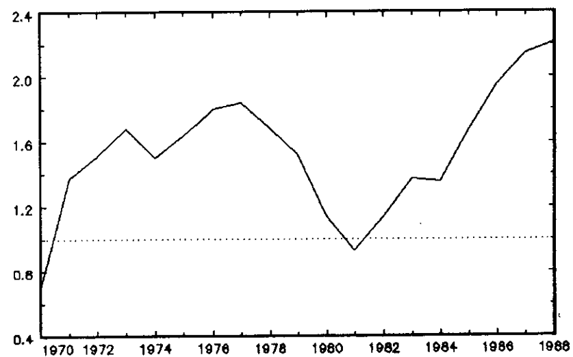
Figure 13(d): Bayes Model Forecast Encompassing Test Statistic: dQ^B/dQ^F
