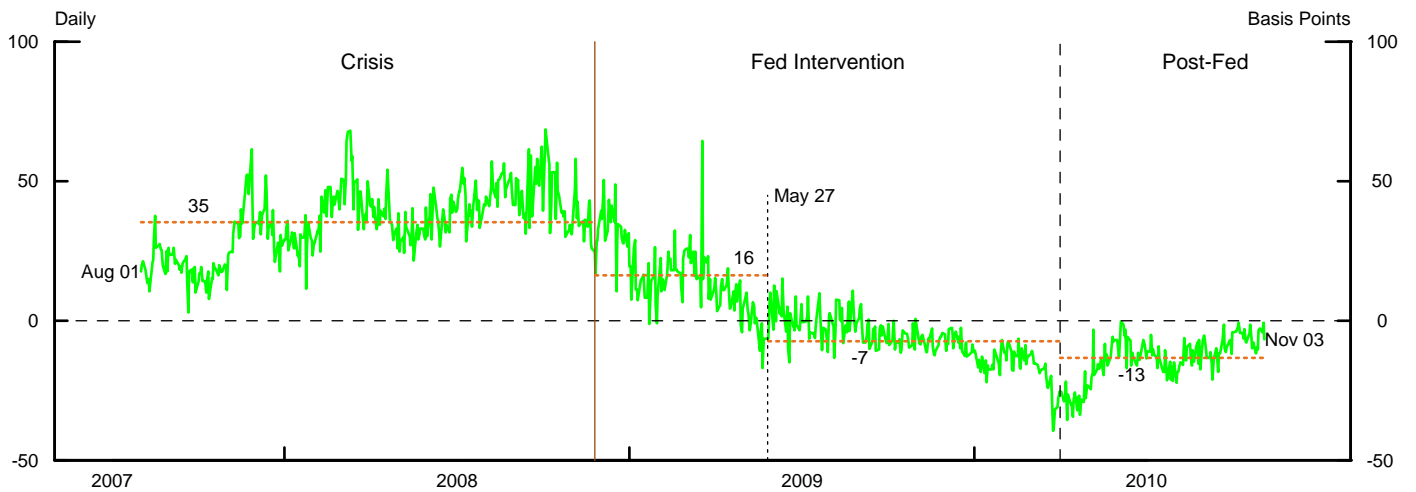
Actual - Predicted Long Swap Rates (After Aug. 1, 2007)
