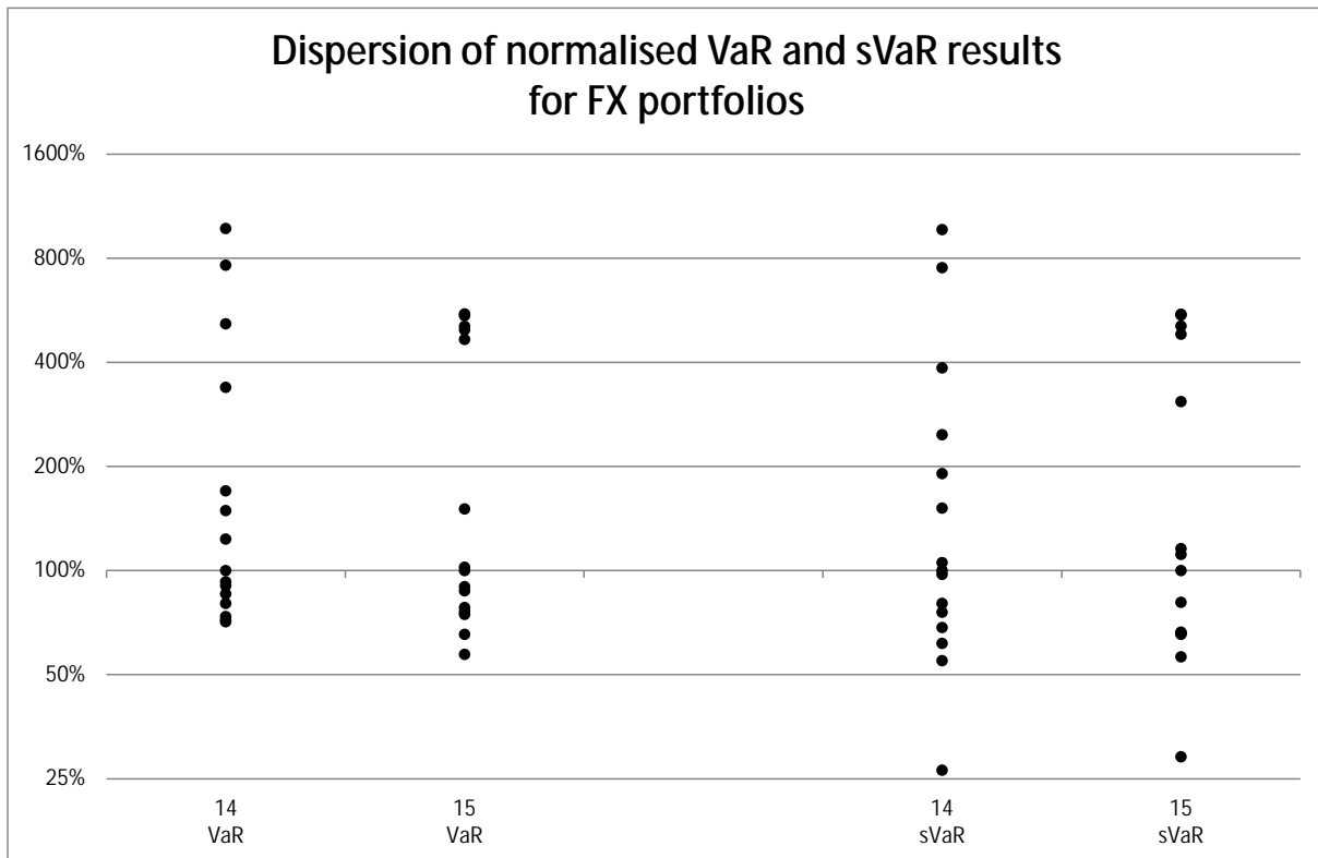
Figure 12: Dispersion of normalised VaR and sVaR for the FX portfolios
