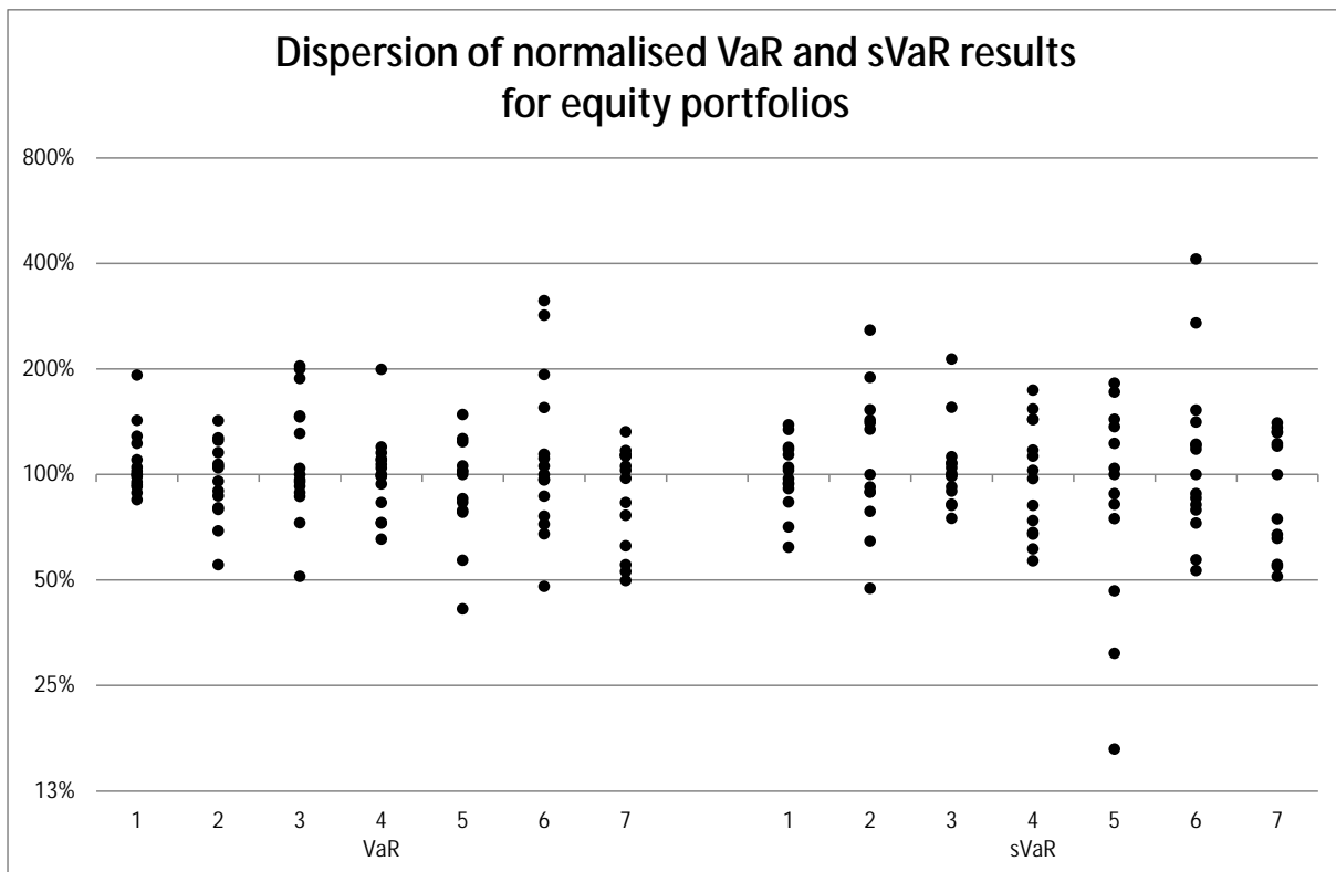
Figure 10: Dispersion of normalised VaR and sVaR for the equity portfolios
