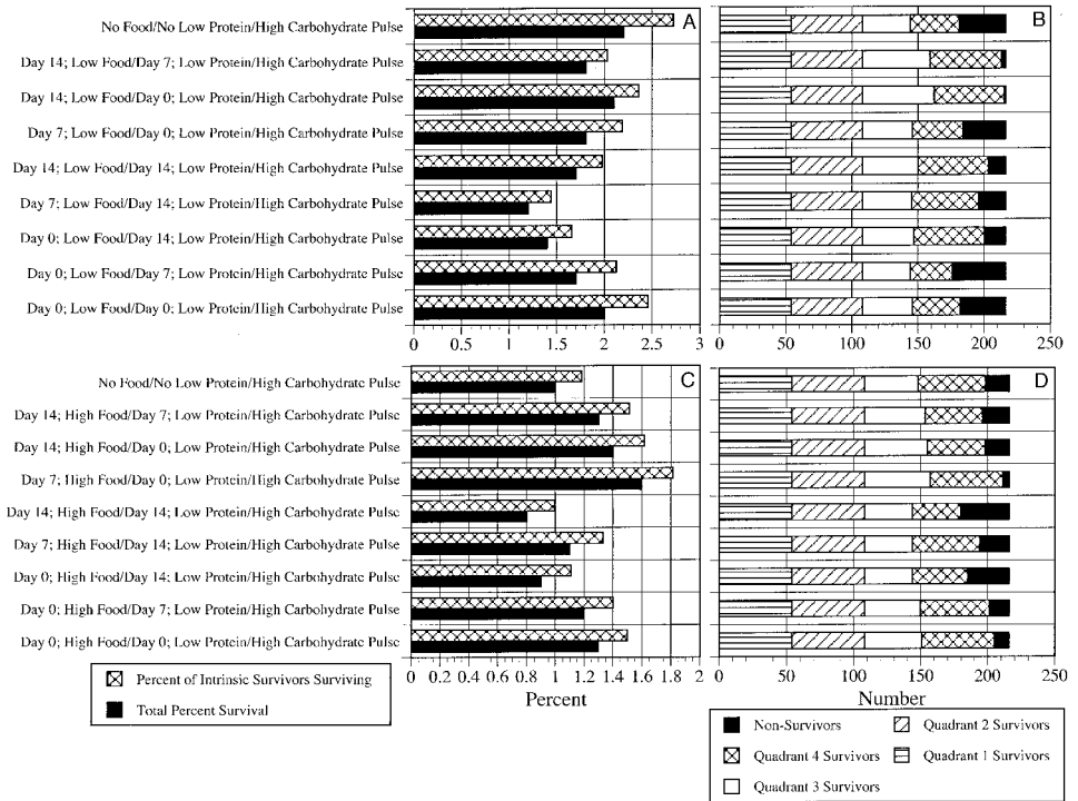
Figure 11. Summary of simulations focusing on short-term variations in the proportion of carbohydrate and protein in the diet and short-term variations in the concentration of food at 27.5‰ and 27.5°C. Time variability in food quality and food concentration was imposed as 7-day events centered on days 0, 7, or 14, as shown in Figure 5. Food concentration varied between 0.5 mg L -1 and 1 mg L -1 . Summary of simulation results expressed as (A, C) the percent of the larval cohort surviving and the percent of intrinsic survivors surviving and (B, D) the number of genetic combinations of egg size and growth efficiency yielding intrinsic survivors. Quadrant definitions: quadrant 1, low growth-efficiency larvae from small eggs; quadrant 2, low growth-efficiency larvae from large eggs; quadrant 3, high growth-efficiency larvae from small eggs; quadrant 4, high growth-efficiency larvae from large eggs. The key to the left indicates the day on which the variation in food quantity was centered, the variation in the food quantity imposed, the day on which the variation in food quality was centered, and the variation in food quality imposed. As an example, case 2 records the results for a simulation in which food quantity was increased for a 7-day period centered on Day 14 and food quality was varied such that carbohydrate increased and protein decreased during a 7-day period centered on Day 7. Results for constant food quality over the larva’s lifetime, designated ‘No’ pulse, are shown in case 1 for comparison. Cases referred to in the text are enumerated with case 1 at the top and case 9 at the bottom.
