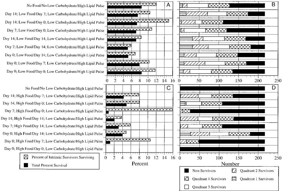
Figure 9. Summary of simulations focusing on short-term variations in the proportion of lipid and carbohydrate in the diet and independent short-term variations in the concentration of food at 27.5‰ and 27.5°C. Time variability in food quality and food concentration was imposed as 7-day events centered on days 0, 7, or 14, as shown in Figure 8. Food concentration varied between 0.5 mg L -1 and 1 mg L -1 . Summary of simulation results expressed as (A, C) the percent of the larval cohort surviving and the percent of intrinsic survivors surviving and (B, D) the number of genetic combinations of egg size and growth efficiency yielding intrinsic survivors. Quadrant definitions: quadrant 1, low growth-efficiency larvae from small eggs; quadrant 2, low growth-efficiency larvae from large eggs; quadrant 3, high growth-efficiency larvae from small eggs; quadrant 4, high growth-efficiency larvae from large eggs. The key to the left indicates the day on which the variation in food quantity was centered, the variation in food quantity imposed, the day on which the variation in food quality was centered, and the variation in food quality imposed. As an example, case 2 records the results for a simulation in which food quantity was increased for a 7-day period centered on Day 14 and food quality was varied such that lipid increased and carbohydrate decreased during a 7-day period centered on Day 7. Results for constant food quality and quantity over the larva’s lifetime, designated ‘No’ pulse, are shown in case 1 for comparison. Cases referred to in the text are enumerated with case 1 at the top and case 9 at the bottom.
