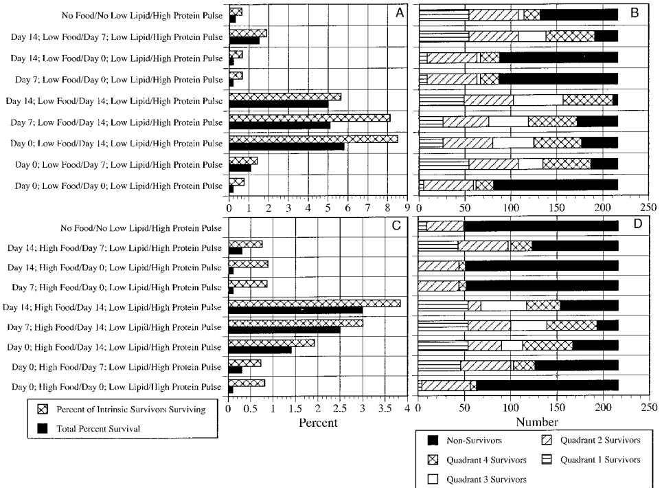
Figure 10. Summary of simulations focusing on short-term variations in the proportion of lipid and protein in the diet and independent short-term variations in the concentration of food at 27.5% and 27.5°C. Time variability in food quality and food concentration was imposed as 7-day events centered on days 0, 7, or 14, as shown in Figure 6. Food concentration varied between 0.5 mg L -1 and 1 mg L -1 . Summary of simulation results expressed as (A, C) the percent of the larval cohort surviving and the percent of intrinsic survivors surviving and (B, D) the number of genetic combinations of egg size and growth efficiency yielding intrinsic survivors. Quadrant definitions: quadrant 1, low growth-efficiency larvae from small eggs; quadrant 2, low growth-efficiency larvae from large eggs; quadrant 3, high growth-efficiency larvae from small eggs; quadrant 4, high growth-efficiency larvae from large eggs. The key to the left indicates the day on which the variation in food quantity was centered, the variation in food quantity imposed, the day on which the variation in food quality was centered, and the variation in food quality imposed. As an example, case 2 records the results for a simulation in which food quantity was increased for a 7-day period centered on Day 14 and food quality was varied such that protein increased and lipid decreased during a 7-day period centered on Day 7. Results for constant food quality over the larva’s lifetime, designated ‘No’ pulse, are shown in case 1 for comparison. Cases referred to in the text are enumerated with case 1 at the top and case 9 at the bottom.
