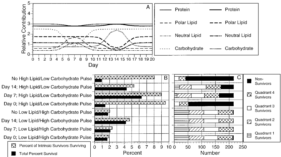
Figure 8. Summary of simulations focusing on short-term variations in the proportion of lipid and carbohydrate in the diet at 27.5‰, 27.5°C, and a 0.75 mg L -1 ration. (A) Time variability in food quality was imposed as 7-day events centered on days 0, 7, or 14. An increase in lipid and decrease in carbohydrate centered on Day 7 (left legend, narrow lines) and an increase in carbohydrate and decrease in lipid centered on Day 14 (right legend, thick lines) are shown. Summary of simulation results expressed as (B) the percent of the larval cohort surviving and the percent of intrinsic survivors surviving and (C) the number of genetic combinations of egg size and growth efficiency yielding intrinsic survivors. Quadrant definitions: quadrant 1, low growth-efficiency larvae from small eggs; quadrant 2, low growth-efficiency larvae from large eggs; quadrant 3, high growth-efficiency larvae from small eggs; quadrant 4, high growth-efficiency larvae from large eggs. The key to the left indicates the day on which the variation in food quality was centered and the variation in food quality imposed. Results for constant food quality over the larva’s lifetime, designated ‘No’ pulse, are shown in cases 1 and 5 for comparison. Cases referred to in the text are enumerated with case 1 at the top and case 8 at the bottom.
