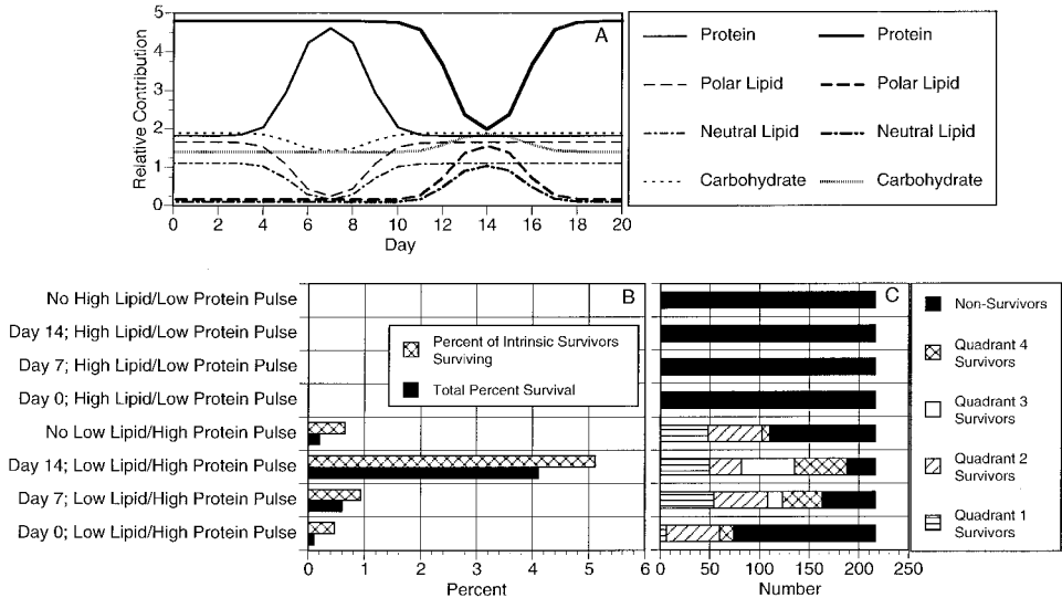
Figure 7. Summary of simulations focusing on short-term variations in the proportion of lipid and protein in the diet at 27.5‰, 27.5°C, and a 0.75 mg L -1 ration. (A) Time variability in food quality was imposed as 7-day events centered on days 0, 7, or 14. An increase in protein and decrease in lipid centered on Day 7 (left legend, narrow lines) and an increase in lipid and decrease in protein centered on Day 14 (right legend, thick lines) are shown. Summary of simulation results expressed as (B) the percent of the larval cohort surviving and the percent of intrinsic survivors surviving and (C) the number of genetic combinations of egg size and growth efficiency yielding intrinsic survivors. Quadrant definitions: quadrant 1, low growth-efficiency larvae from small eggs; quadrant 2, low growth-efficiency larvae from large eggs; quadrant 3, high growth-efficiency larvae from small eggs; quadrant 4, high growth-efficiency larvae from large eggs. The key to the left indicates the day on which the variation in food quality was centered and the variation in food quality imposed. Results for constant food quality over the larva's lifetime, designated 'No' pulse, are shown in cases 1 and 5 for comparison. Cases referred to in the text are enumerated with case 1 at the top and case 8 at the bottom.
