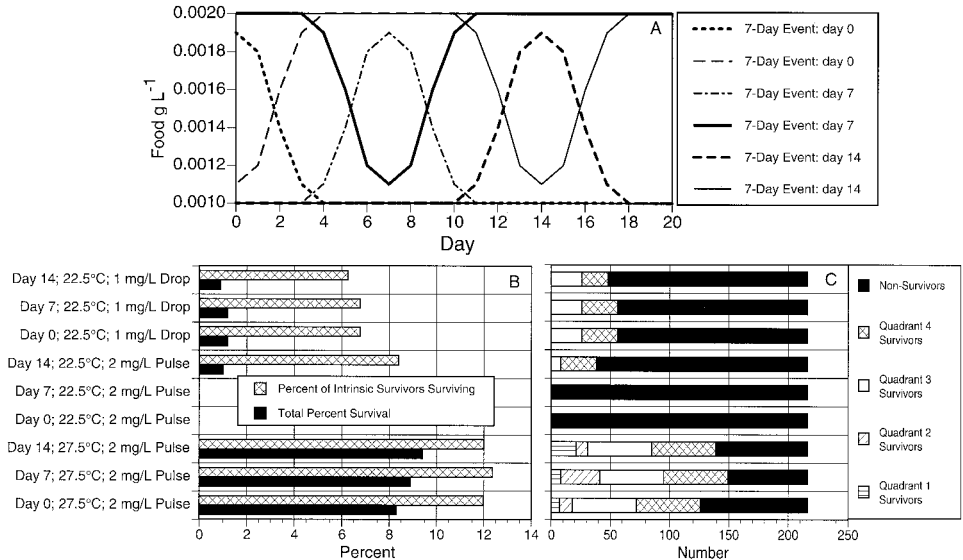
Figure 2. Results of simulations focusing on short-term variations in food concentration obtained for 27.5% and a ration of standard food at 27.5°C and 22.5°C. (A) Time variability of food concentration was imposed as 7-day events centered on days 0, 7, or 14, during which time food concentration increased from 1 mg L -1 to 2 mg L -1 or decreased from 2 mg L -1 to 1 mg L -1 . Time series are in pairs, with the first in each pair a 7-d increase in food and the second in each pair a 7-d decrease in food. Summary of simulation results expressed as (B) the percent of the larval cohort surviving and the percent of intrinsic survivors surviving and (C) the number of genetic combinations of egg size and growth efficiency yielding intrinsic survivors. Quadrant definitions: quadrant 1, low growth-efficiency larvae from small eggs; quadrant 2, low growth-efficiency larvae from large eggs; quadrant 3, high growth-efficiency larvae from small eggs; quadrant 4, high growth-efficiency larvae from large eggs. The key to the left indicates the day on which the food pulse was centered (e.g., Day 14), the temperature used for the simulation (e.g., 22°C) and the magnitude and type of food variation used (e.g., a 1 mg L -1 decline). Cases referred to in the text are enumerated with case 1 at the top and case 9 at the bottom.
