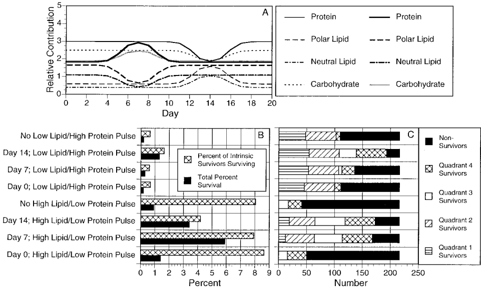
Figure 6. Results of simulations focusing on short-term variations in the proportion of lipid and protein in the diet at 27.5‰, 27.5°C, and a 0.75 mg L -1 ration. (A) Time variability in food quality was imposed as 7-day events centered on days 0, 7, or 14. An increase in protein and decrease in lipid centered on Day 7 (right legend, thick lines) and an increase in lipid and decrease in protein centered on Day 14 (left legend, thin lines) are shown. Summary of simulation results expressed as (B) the percent of the larval cohort surviving and the percent of intrinsic survivors surviving and (C) the number of genetic combinations of egg size and growth efficiency yielding intrinsic survivors. Quadrant definitions: quadrant 1, low growth-efficiency larvae from small eggs; quadrant 2, low growth-efficiency larvae from large eggs; quadrant 3, high growth-efficiency larvae from small eggs; quadrant 4, high growth-efficiency larvae from large eggs. The key to the left indicates the day on which the variation in food quality was centered (e.g., Day 14) and the variation in food quality imposed (e.g., a low lipid, high protein pulse). Results for constant food quality over the larva’s lifetime, designated ‘No’ pulse, are shown in cases 1 and 5 for comparison. Cases referred to in the text are enumerated with case 1 at the top and case 8 at the bottom.
