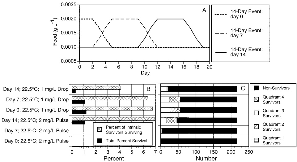
Figure 3. Results of simulations focusing on short-term variations in food concentration obtained for 27.5‰ and a ration of standard food at 27.5°C and 22.5°C. (A) Time variability of food concentration was imposed as 14-day events centered on days 0, 7, or 14, during which time food concentration increased from 1 mg L -1 to 2 mg L -1 or decreased (not shown) from 2 mg L -1 to 1 mg L -1 . Summary of simulation results expressed as (B) the percent of the larval cohort surviving and the percent of intrinsic survivors surviving and (C) the number of genetic combinations of egg size and growth efficiency yielding intrinsic survivors. Quadrant definitions: quadrant 1, low growth-efficiency larvae from small eggs; quadrant 2, low growth-efficiency larvae from large eggs; quadrant 3, high growth-efficiency larvae from small eggs; quadrant 4, high growth-efficiency larvae from large eggs. The key to the left indicates the day on which the food pulse was centered (e.g., Day 14), the temperature used for the simulation (e.g., 22.5°C), and the magnitude and type of food variation used (e.g., 1 mg L -1 decline). Cases referred to in the text are enumerated with case 1 at the top and case 6 at the bottom.
